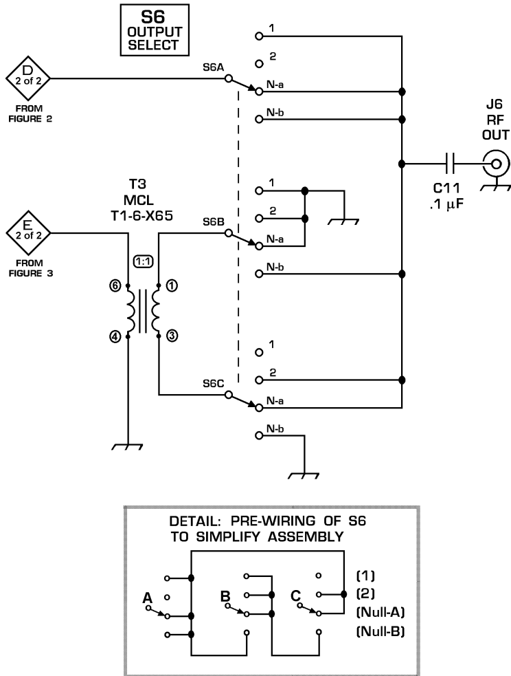
FIGURE 5: MWDX-6 OUTPUT SECTION
