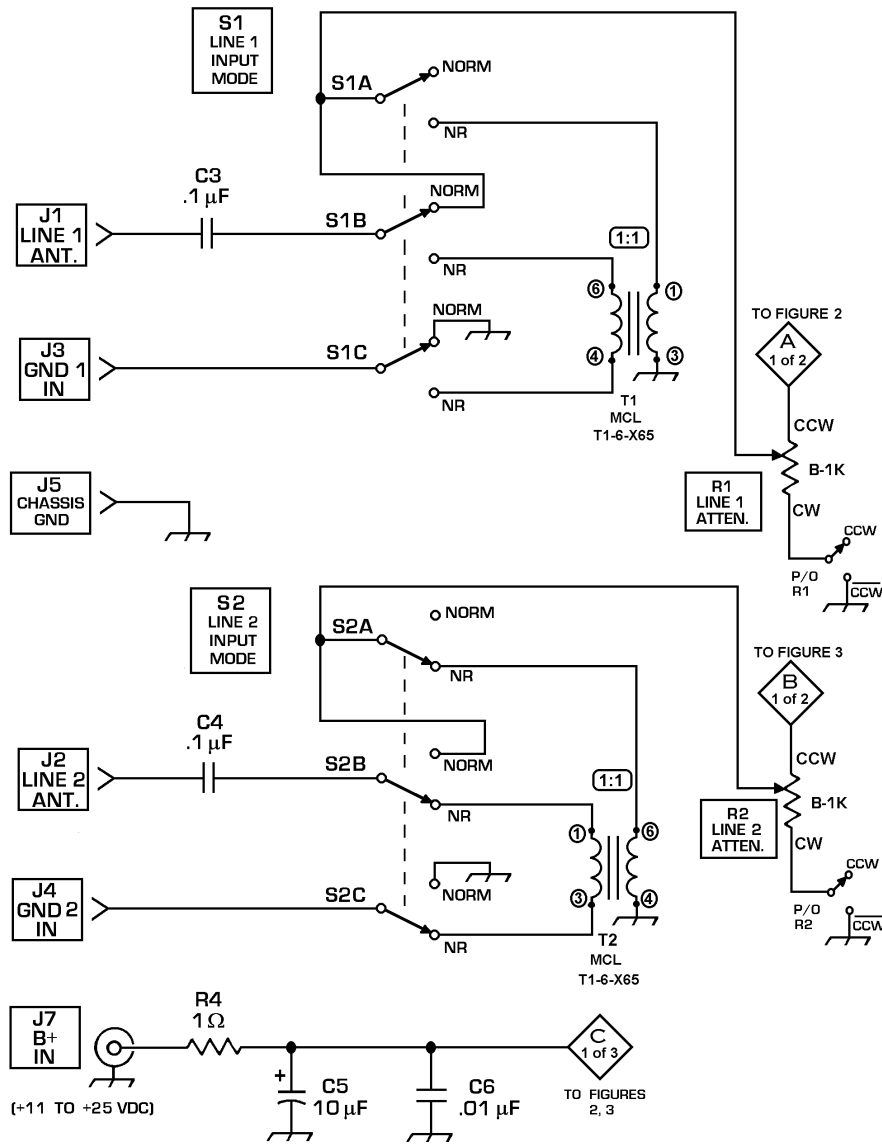
FIGURE 1: MWDX-6 INPUT SECTION SCHEMATIC
