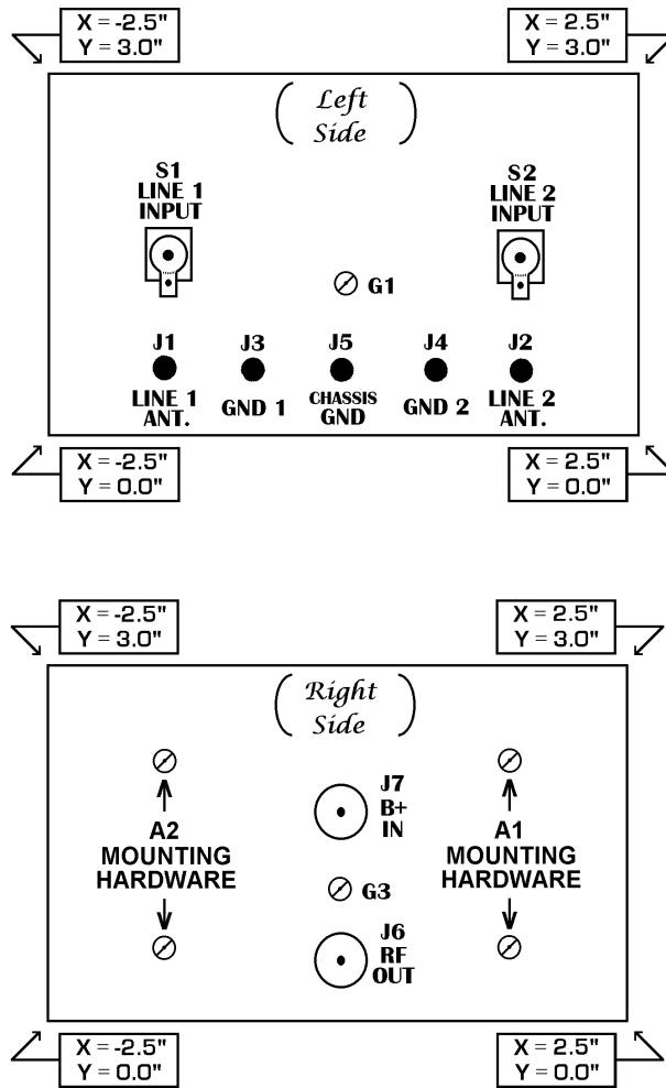
FIGURE 7: MWDX-6 CHASSIS PICTORIALS (LEFT, RIGHT SIDES)
