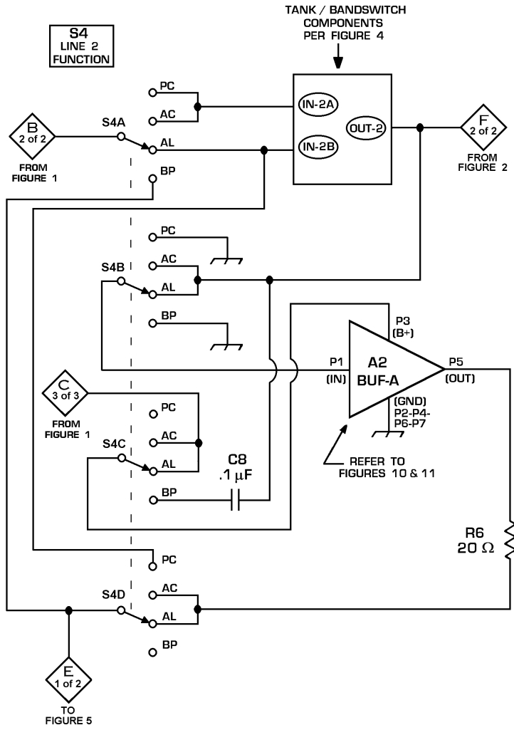
FIGURE 3: MWDX-6 CENTRAL SECTION SCHEMATIC (LINE 2)
