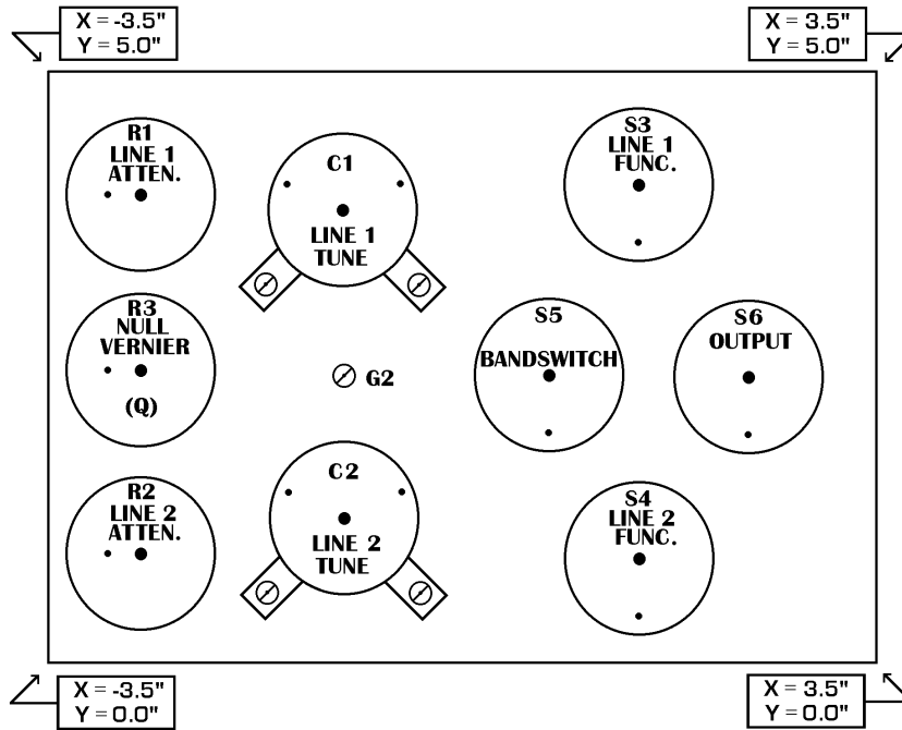
FIGURE 6: MWDX-6 CHASSIS PICTORIAL (TOP)
