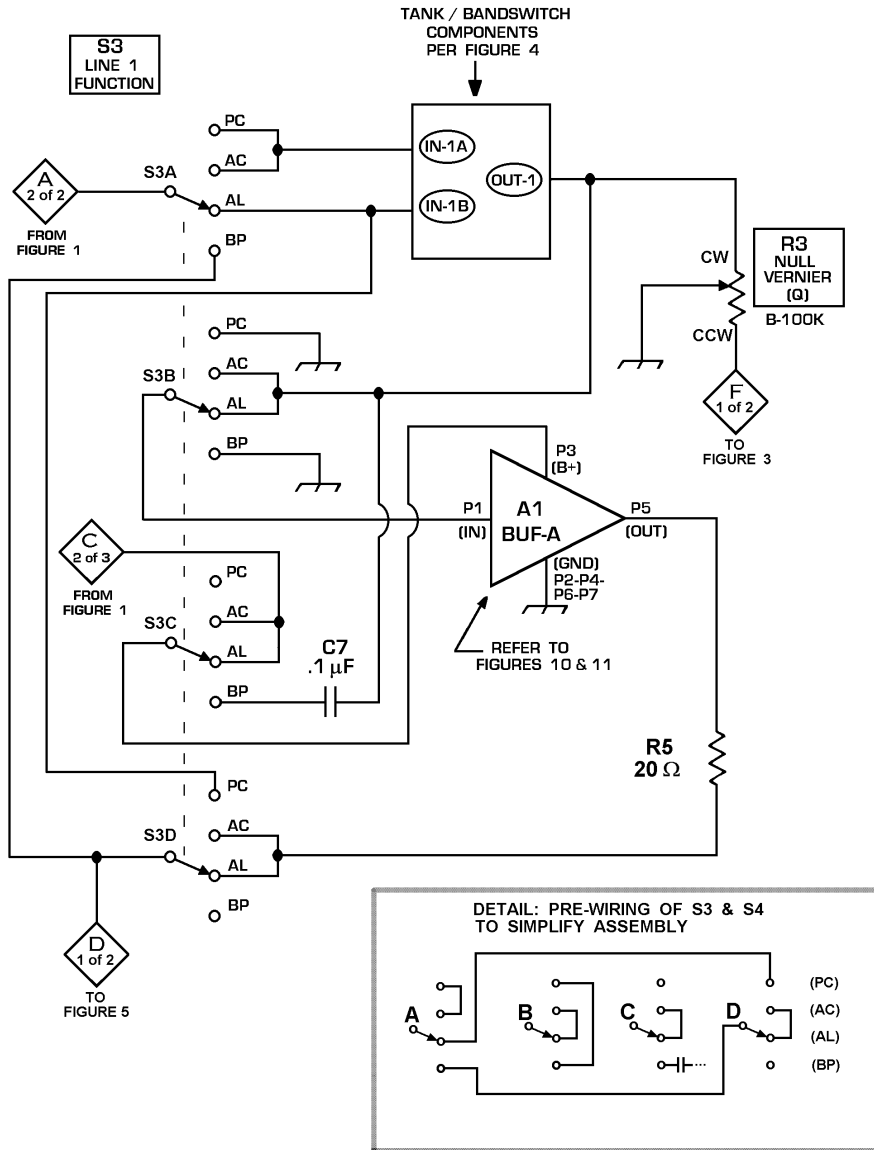
FIGURE 2: MWDX-6 CENTRAL SECTION SCHEMATIC (LINE 1)
