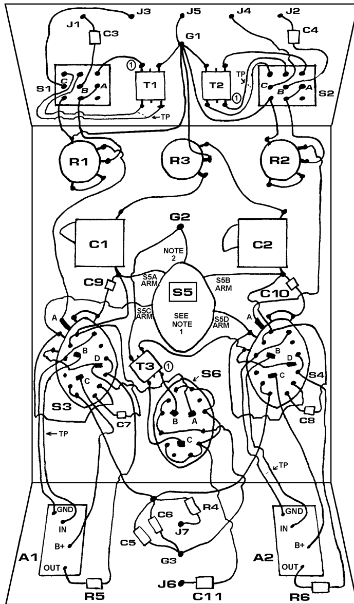
FIGURE 8 MWDX-6 ASSEMBLY PICTORIAL (NOT TO SCALE)
